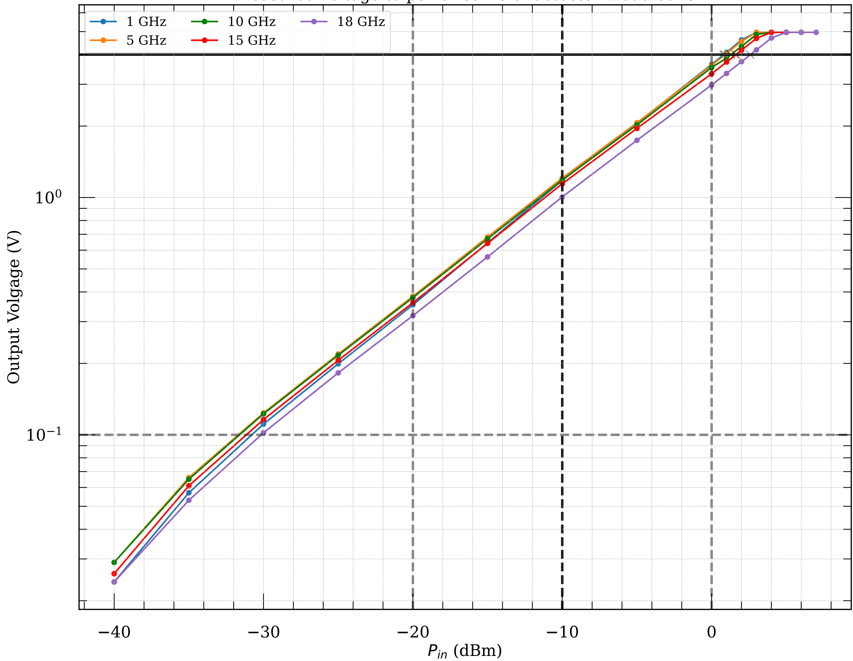
Measured voltage-to-power curve of detector module048
